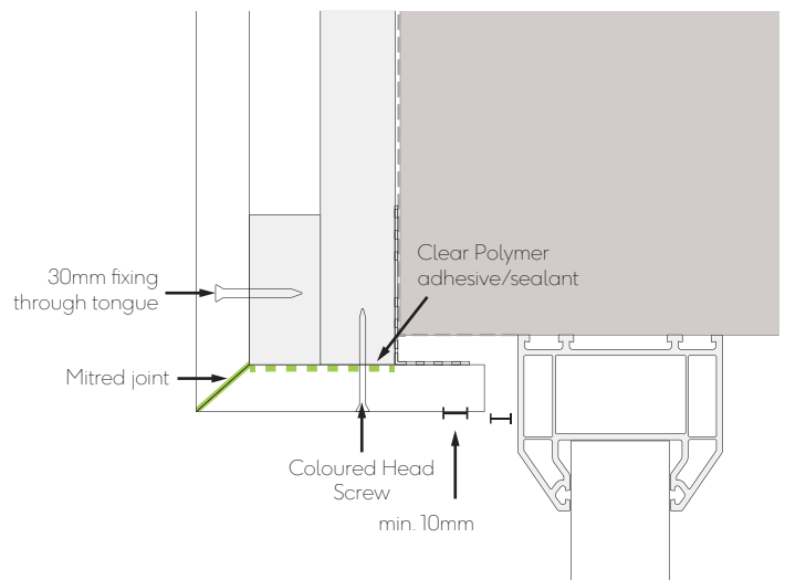
Fig. 14 - Window/door head with mitred joint
